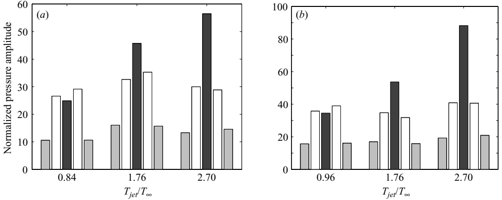
FIGURE 20. Balance of instability-wave amplitude at the peak for different temperature ratios (at St = 0.30 ). (a) M_\infty = 0.9 (cases D, F and H). (b) M_\infty = 0.5 (cases B, E and G). Pressure amplitude of m = 0 for the unheated case at (x/D, r/D) = (0, 0.5) is taken to be unity. Notation is the same as figure 16(b).
